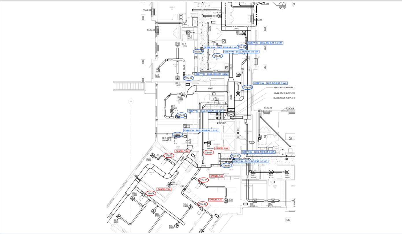
Mark-up M2013 AL area D - bistro, parlor, reception, corridor, activity rooms
